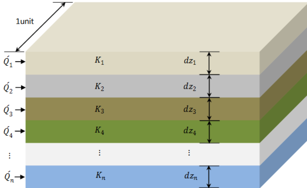
Figure 3: Horizontal Equivalent Hydraulic Conductivity
